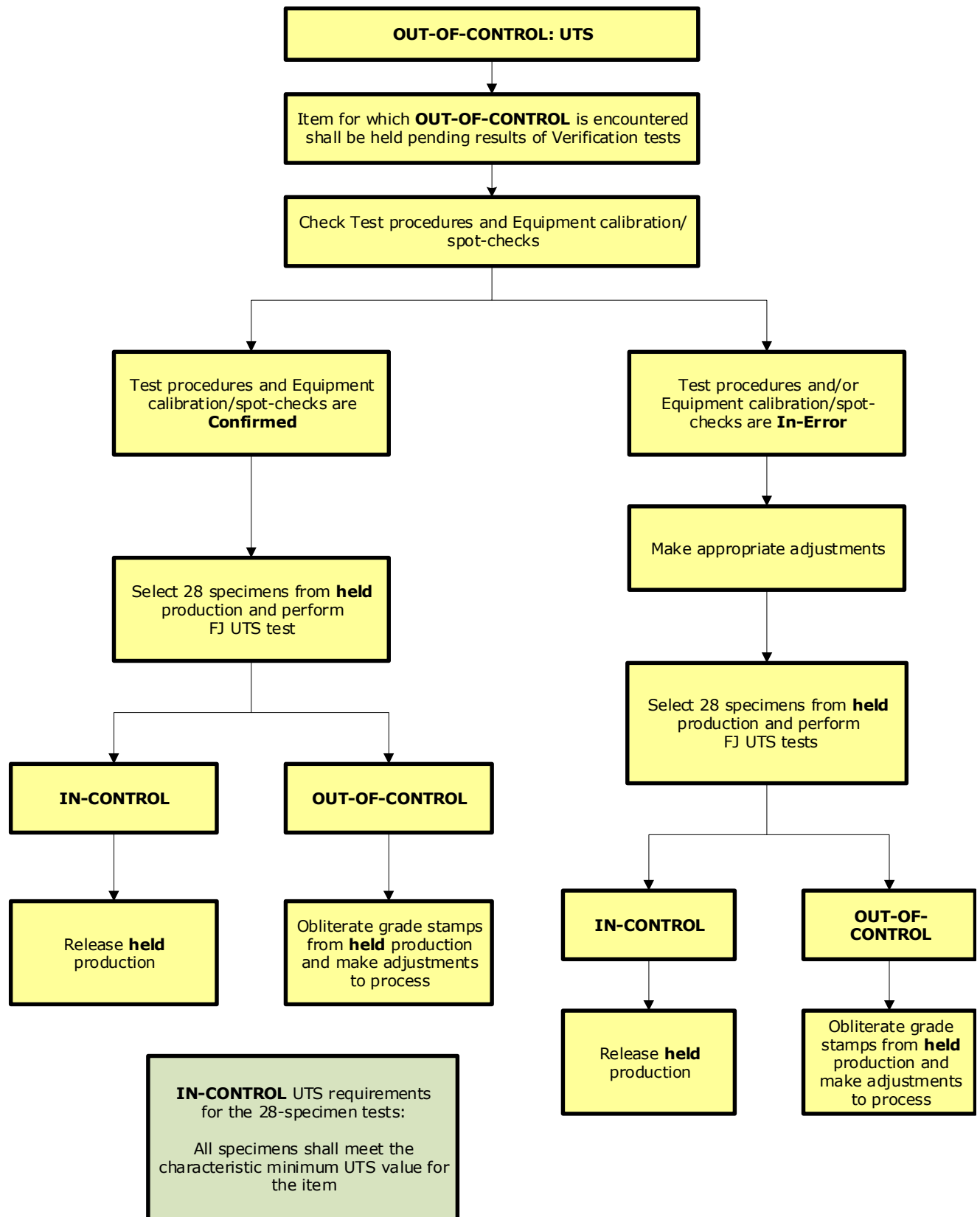
FIGURE 13 – UTS FINGERJOINT VERIFICATION – DECISION FLOW CHART
