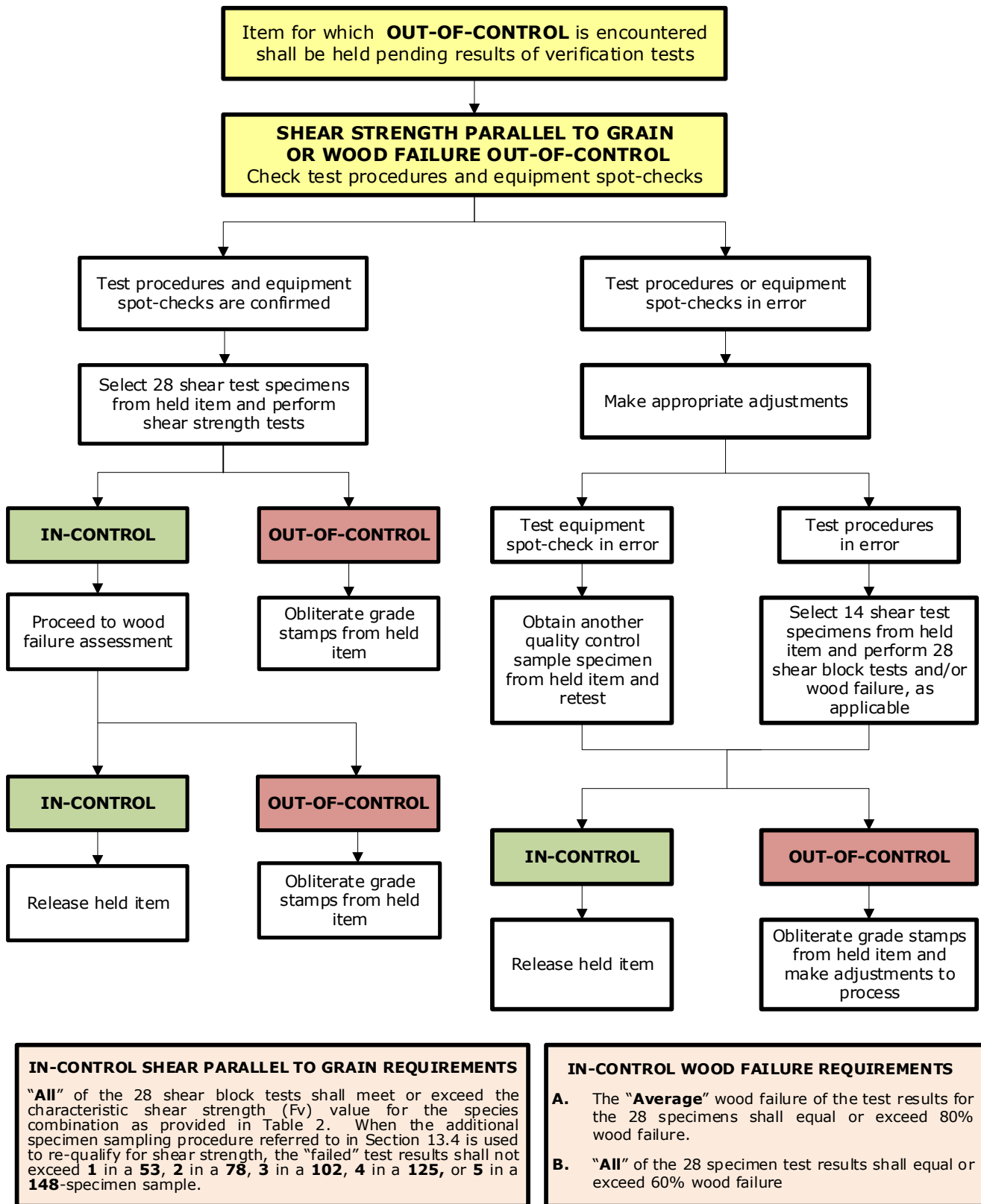
FIGURE 4 - SHEAR STRENGTH PARALLEL TO GRAIN AND/OR WOOD FAILURE RE-QUALIFICATION FLOW CHART
