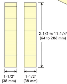
FIGURE 1 - EXAMPLES OF STRUCTURAL FACE-GLUED LUMBER PRODUCT CROSS-SECTIONS
