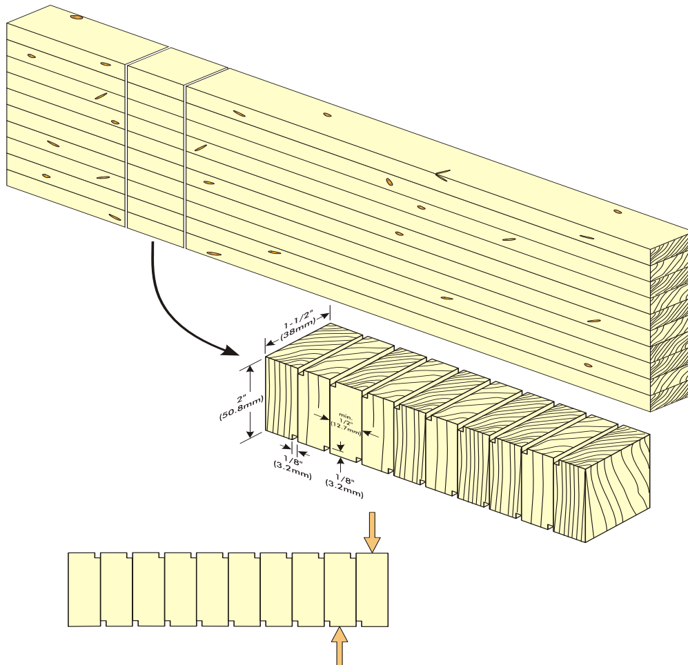
FIGURE 2 - TEST SPECIMEN SHEAR BLOCK AND SAW KERF DIMENSIONS
